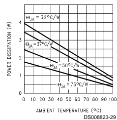
Maximum Power Dissipation (TO-263) (Note 3)
